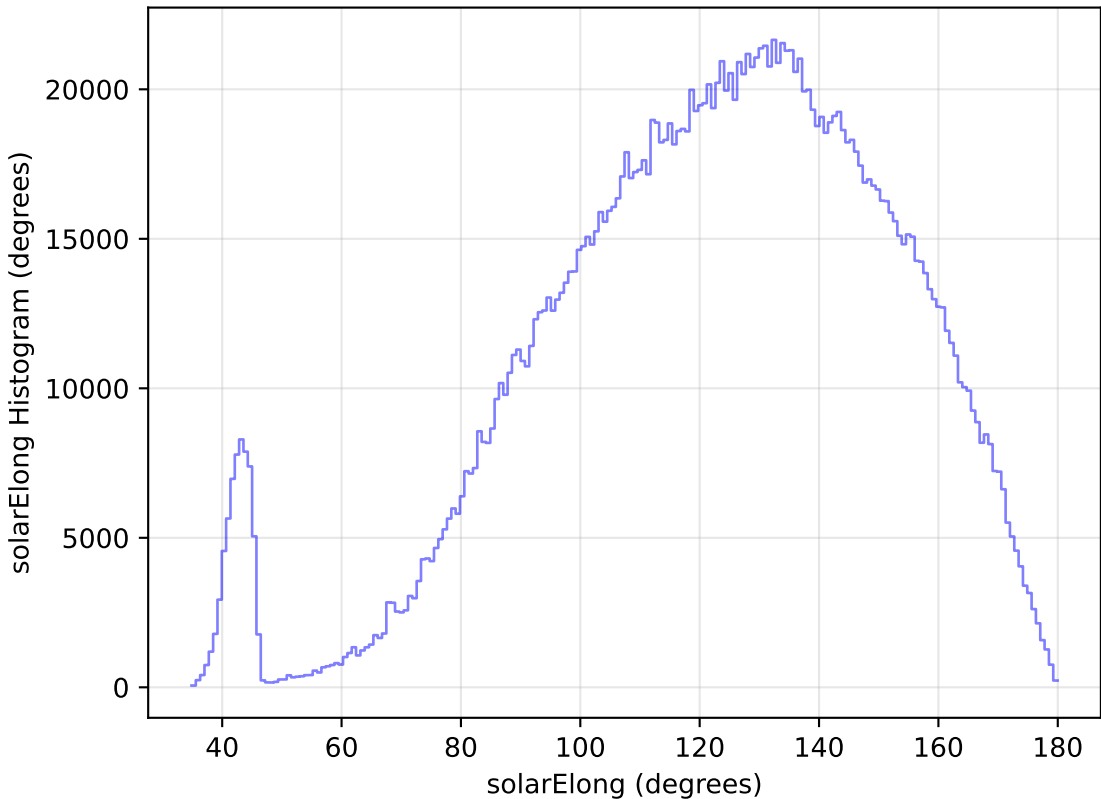
mw_roll_all_v3.3_10yrs WFD all bands: solarElong Histogram
