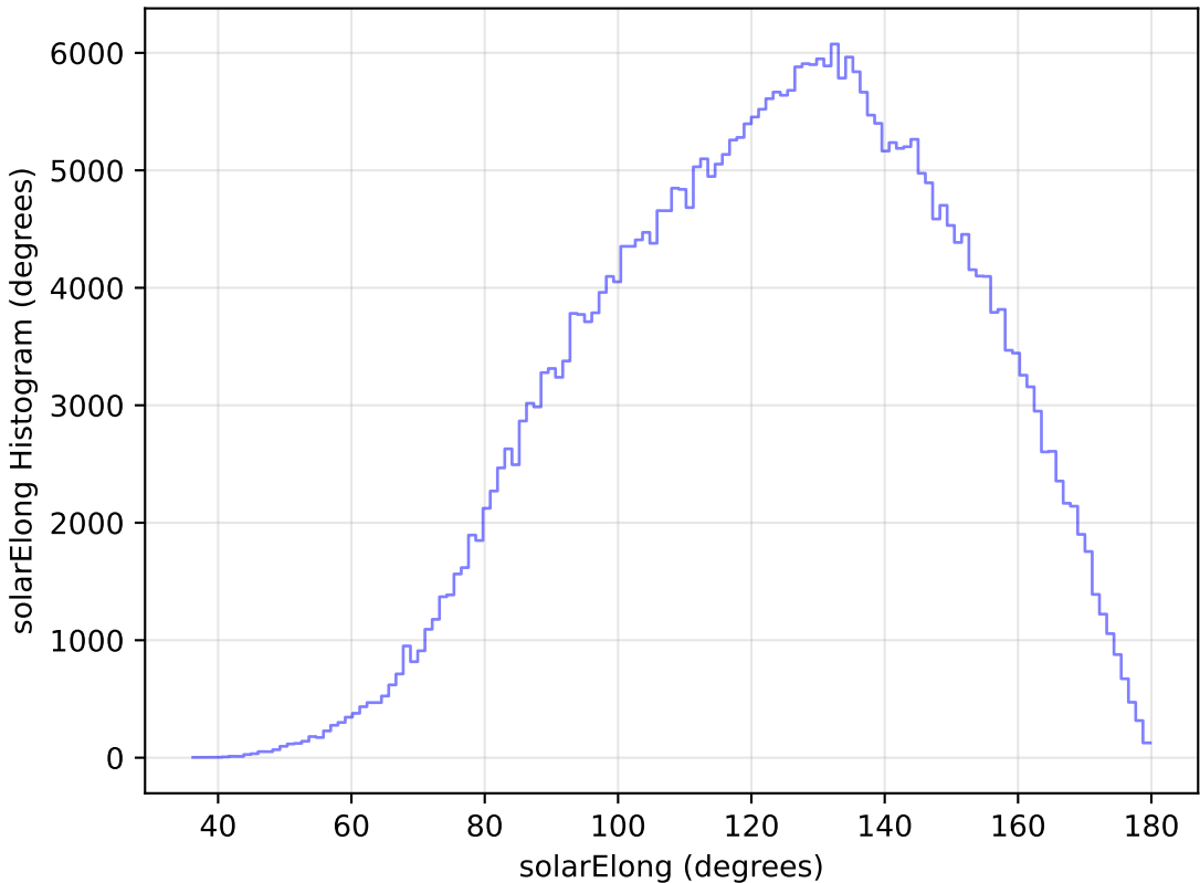
mw_roll_all_v3.3_10yrs All sky y band: solarElong Histogram
