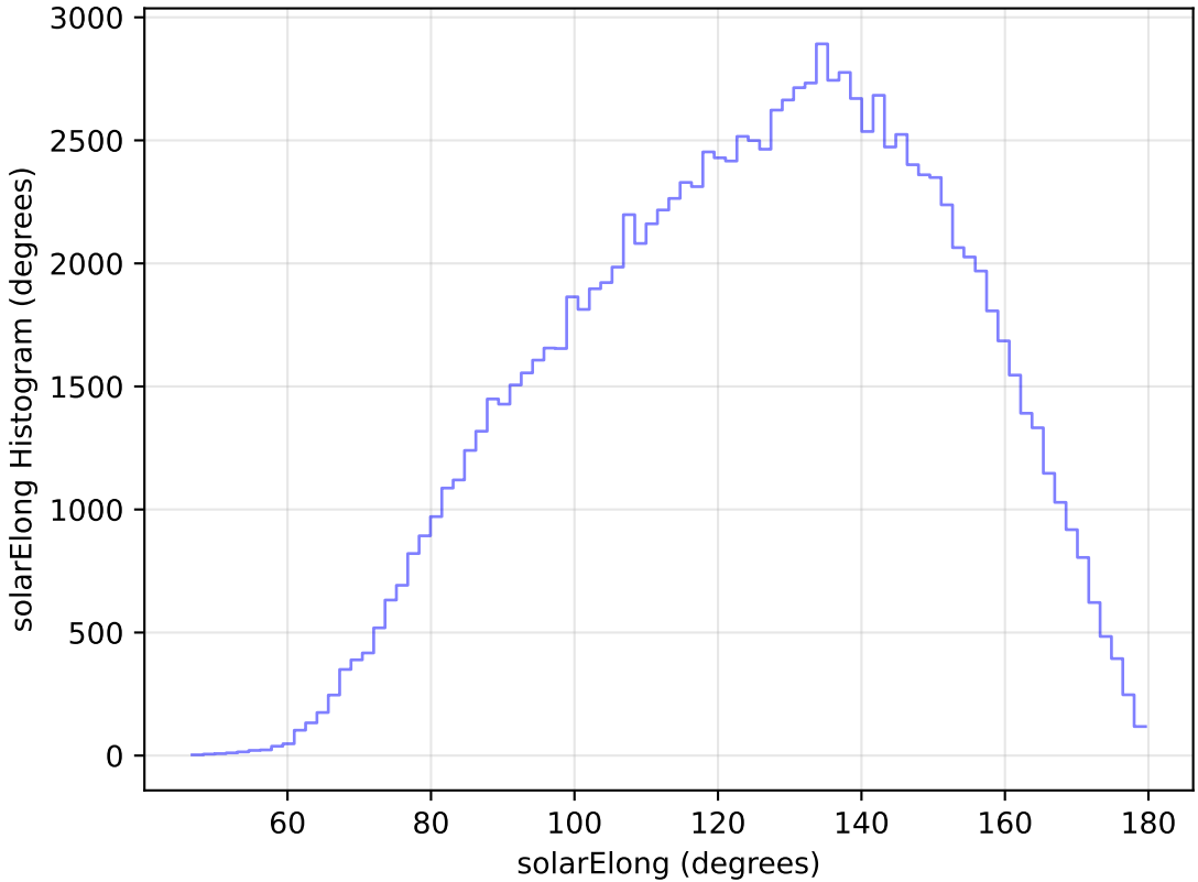
mw_roll_all_v3.3_10yrs All sky u band: solarElong Histogram
