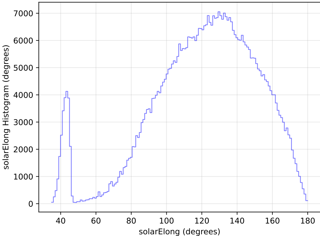
mw_roll_all_v3.3_10yrs All sky i band: solarElong Histogram
