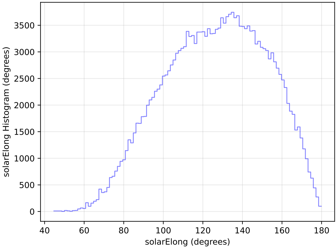
mw_roll_all_v3.3_10yrs All sky g band: solarElong Histogram
