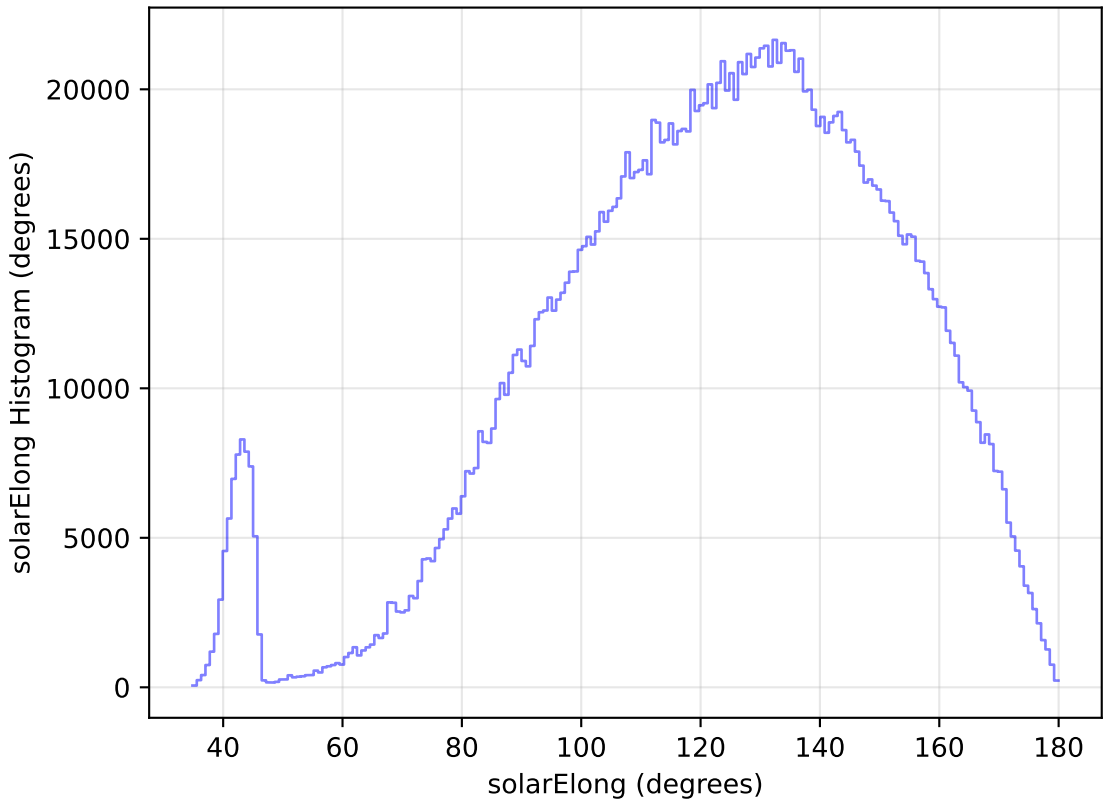
mw_roll_all_v3.3_10yrs All sky all bands: solarElong Histogram
