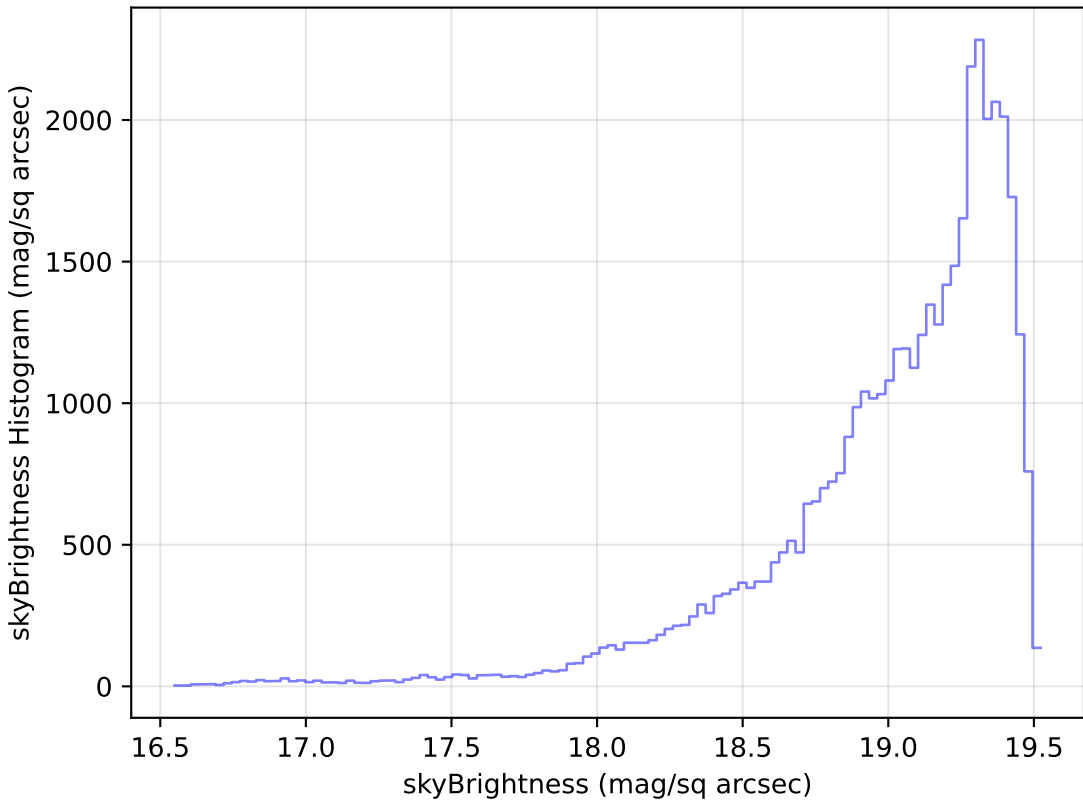
mw_roll_all_v3.3_10yrs Yr 1 z band: skyBrightness Histogram
