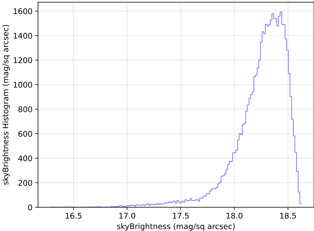
mw_roll_all_v3.3_10yrs Yr 1 y band: skyBrightness Histogram
