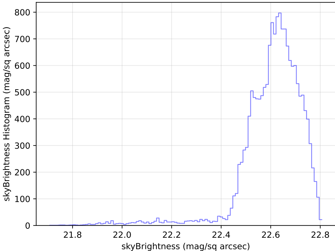
mw_roll_all_v3.3_10yrs Yr 1 u band: skyBrightness Histogram
