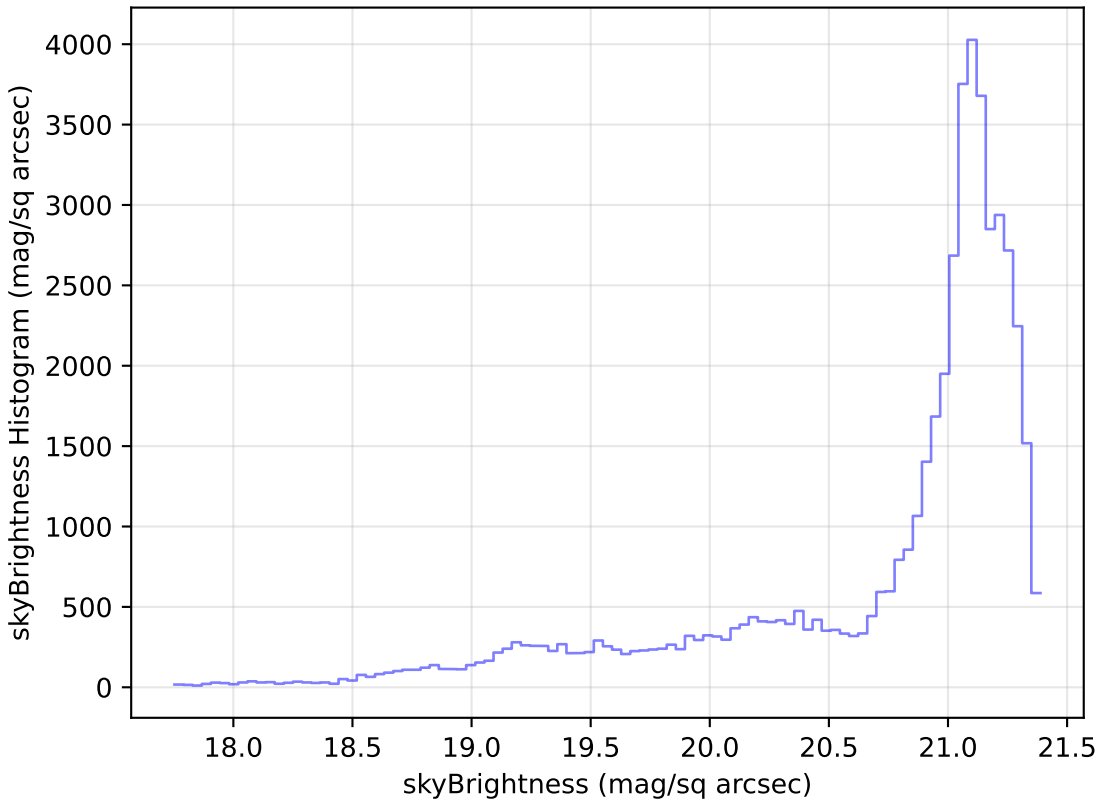
mw_roll_all_v3.3_10yrs Yr 1 r band: skyBrightness Histogram
