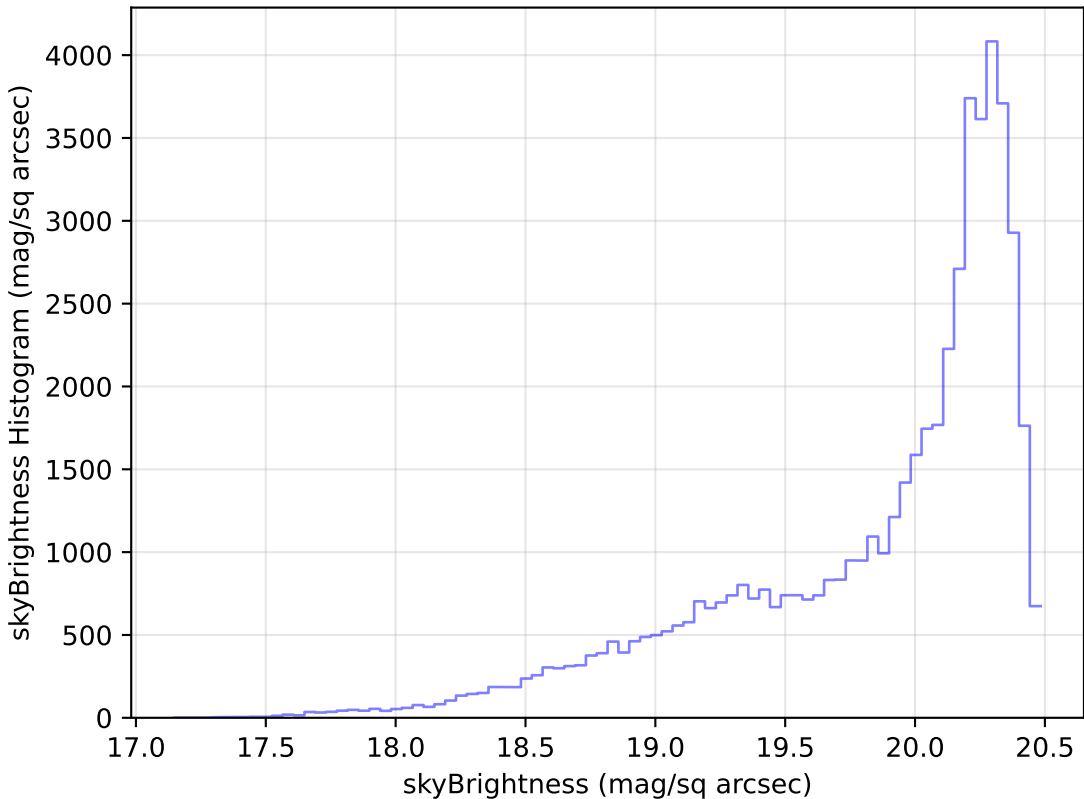
mw_roll_all_v3.3_10yrs Yr 1 i band: skyBrightness Histogram
