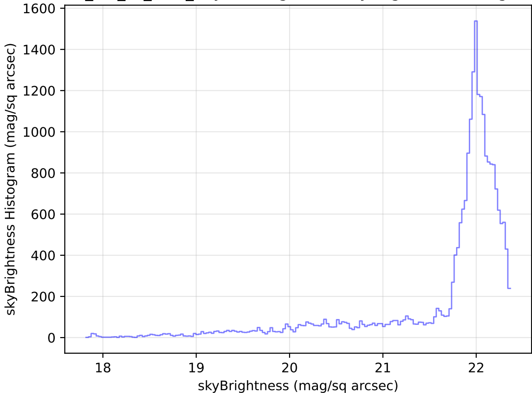
mw_roll_all_v3.3_10yrs Yr 1 g band: skyBrightness Histogram
