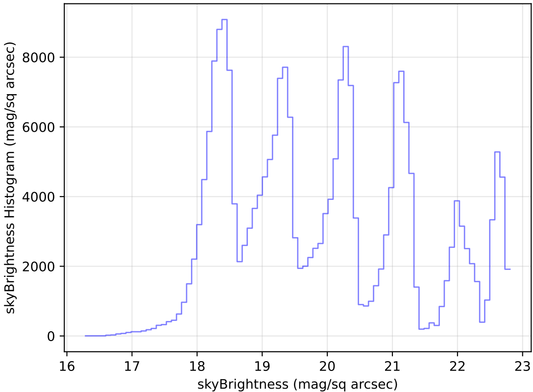
mw_roll_all_v3.3_10yrs Yr 1 all bands: skyBrightness Histogram
