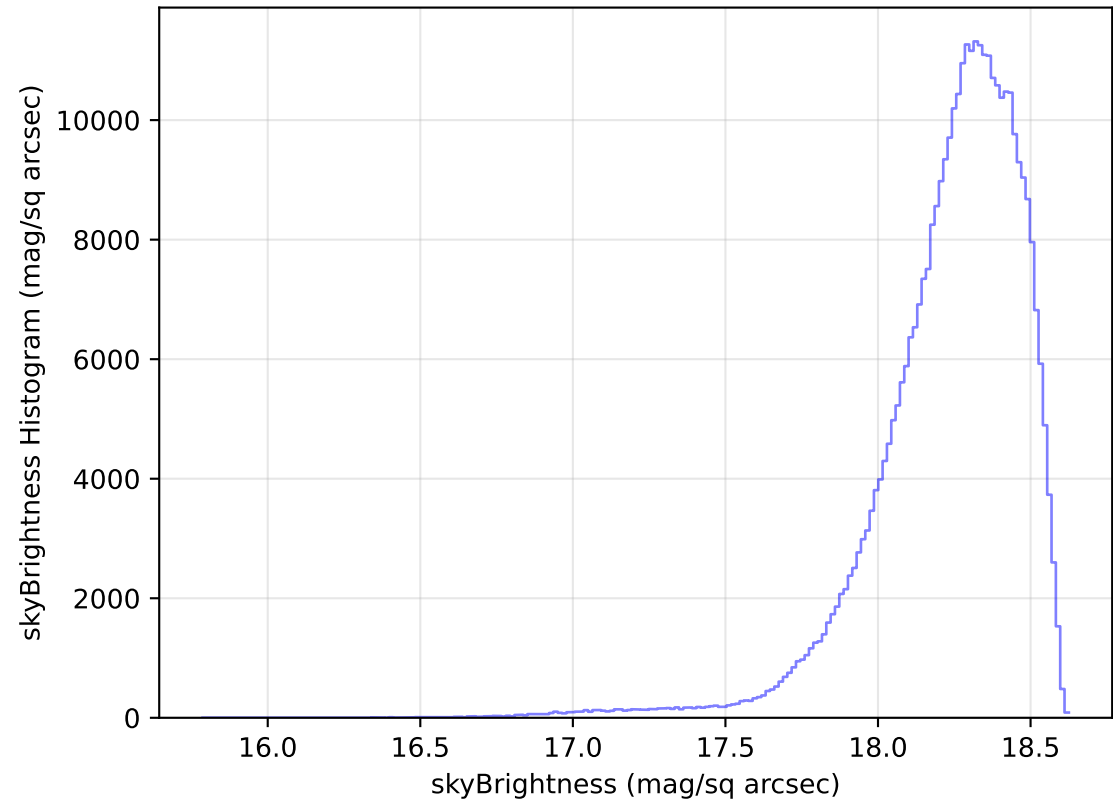
mw_roll_all_v3.3_10yrs WFD y band: skyBrightness Histogram
