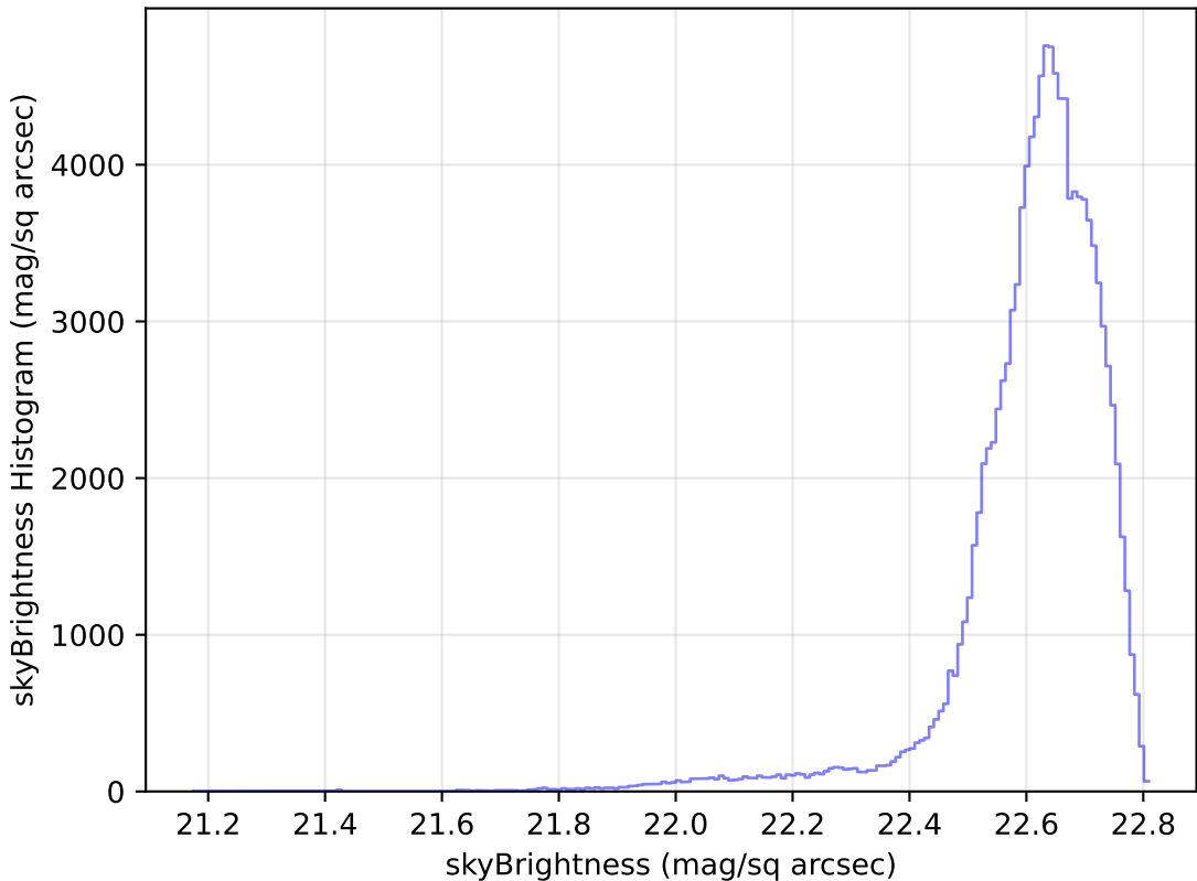
mw_roll_all_v3.3_10yrs WFD u band: skyBrightness Histogram
