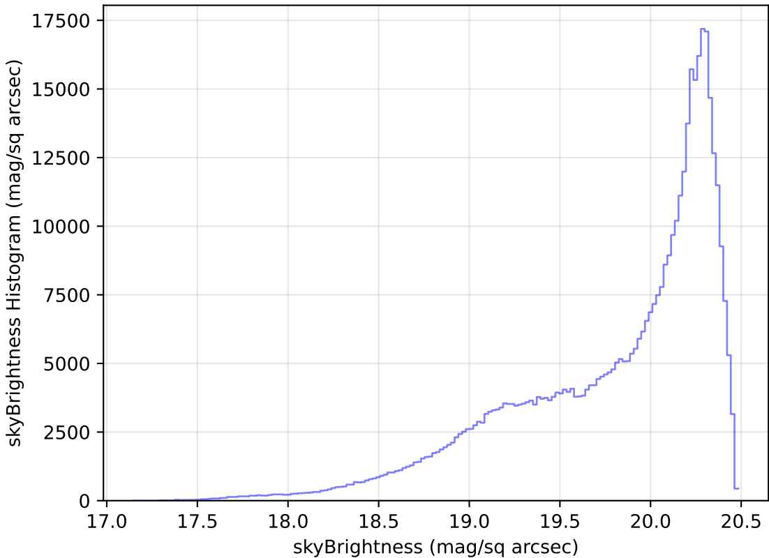
mw_roll_all_v3.3_10yrs WFD i band: skyBrightness Histogram
