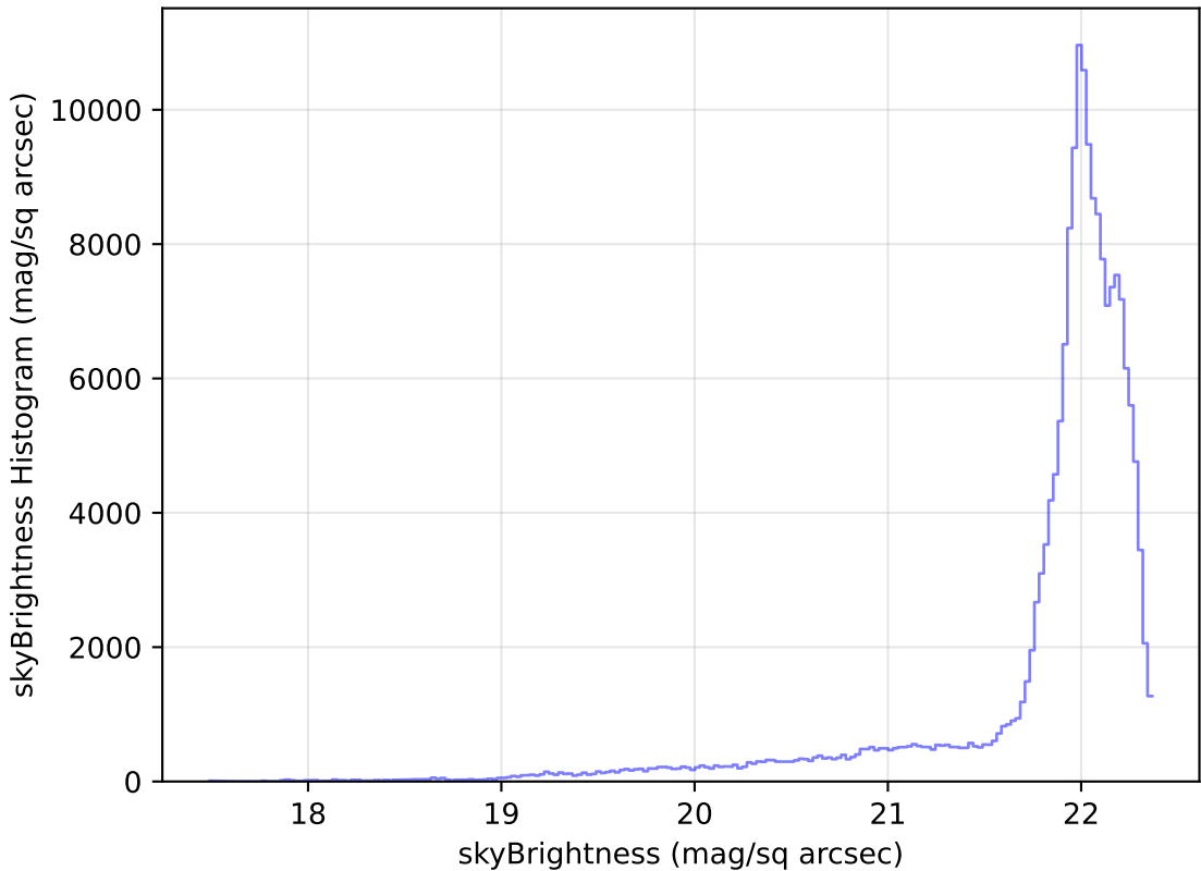
mw_roll_all_v3.3_10yrs WFD g band: skyBrightness Histogram
