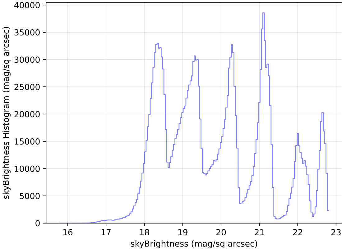
mw_roll_all_v3.3_10yrs WFD all bands: skyBrightness Histogram
