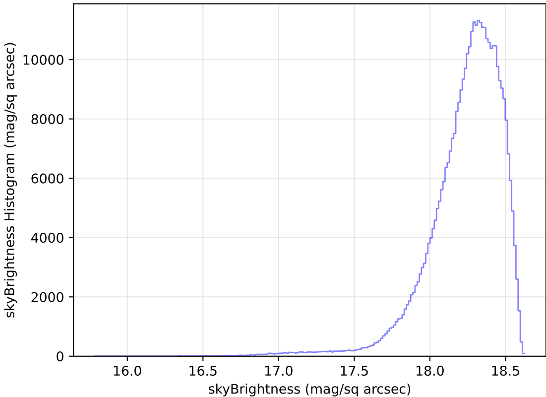
mw_roll_all_v3.3_10yrs All sky y band: skyBrightness Histogram
