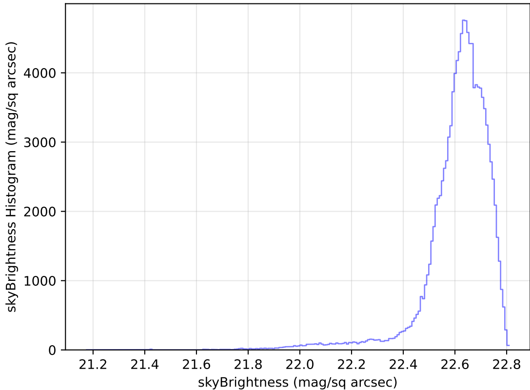
mw_roll_all_v3.3_10yrs All sky u band: skyBrightness Histogram
