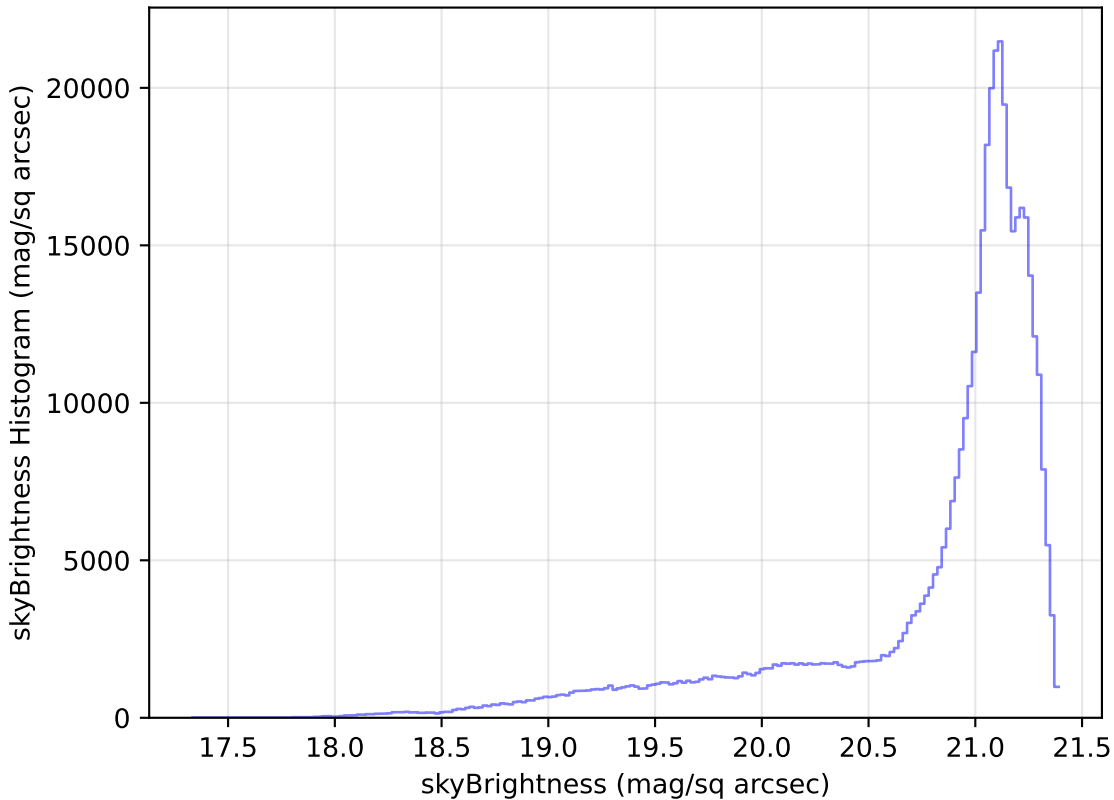
mw_roll_all_v3.3_10yrs All sky r band: skyBrightness Histogram
