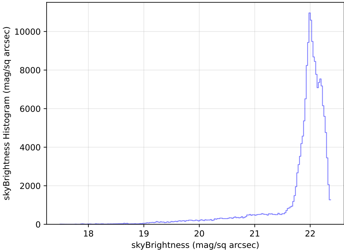
mw_roll_all_v3.3_10yrs All sky g band: skyBrightness Histogram
