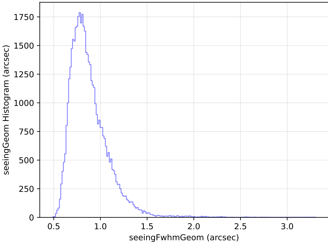
mw_roll_all_v3.3_10yrs Yr 1 y band: seeingGeom Histogram
