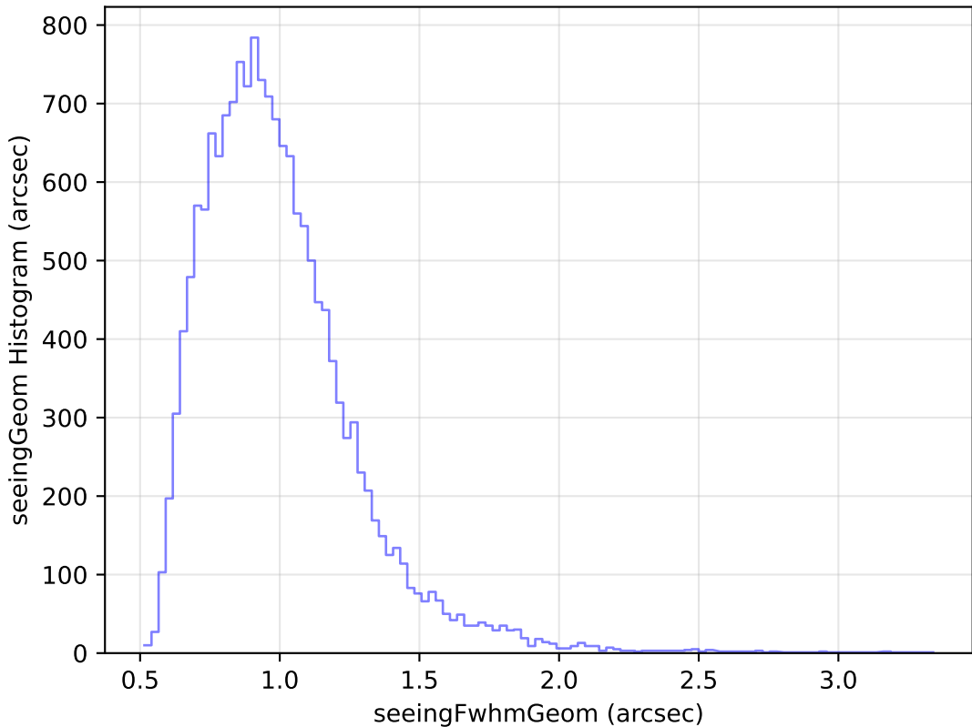
mw_roll_all_v3.3_10yrs Yr 1 u band: seeingGeom Histogram
