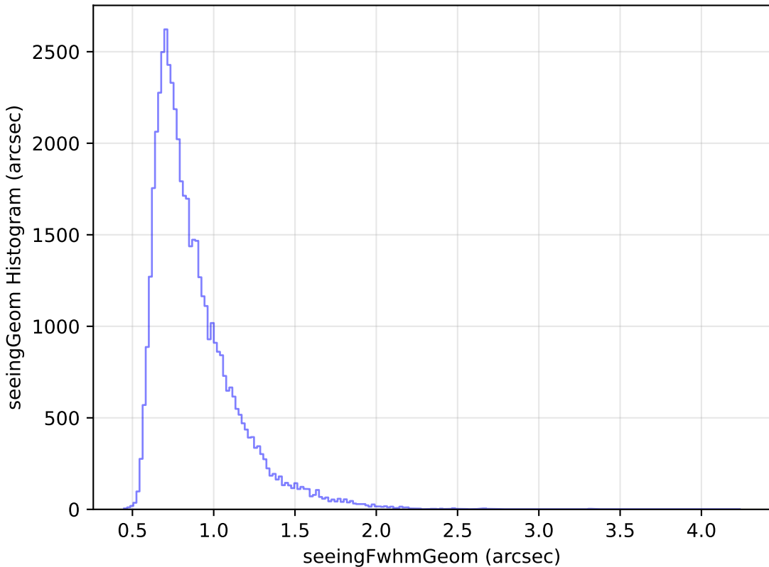
mw_roll_all_v3.3_10yrs Yr 1 r band: seeingGeom Histogram
