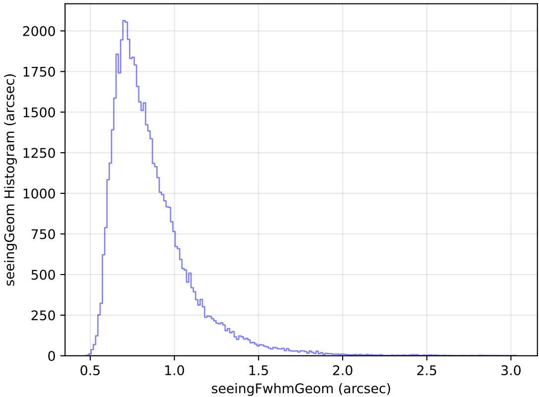
mw_roll_all_v3.3_10yrs Yr 1 i band: seeingGeom Histogram
