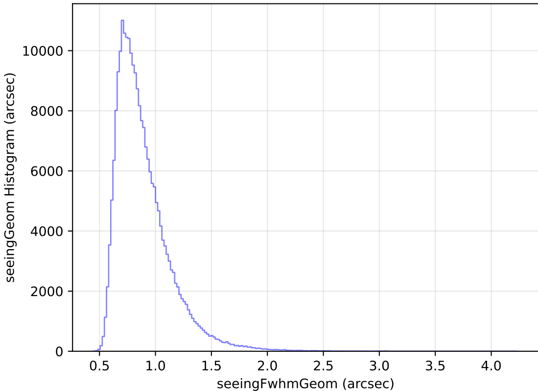
mw_roll_all_v3.3_10yrs Yr 1 all bands: seeingGeom Histogram
