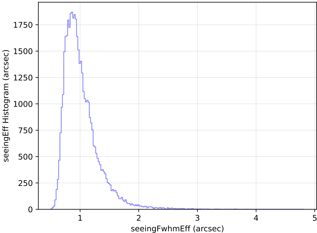
mw_roll_all_v3.3_10yrs Yr 1 z band: seeingEff Histogram
