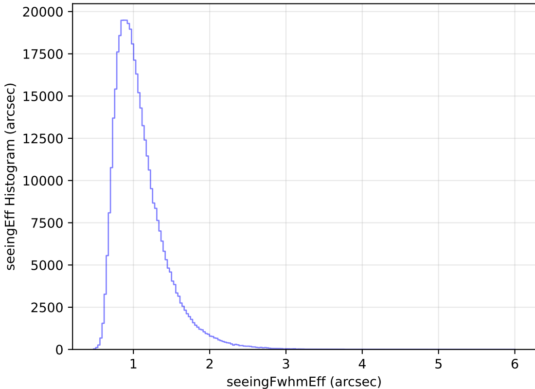
mw_roll_all_v3.3_10yrs WFD z band: seeingEff Histogram
