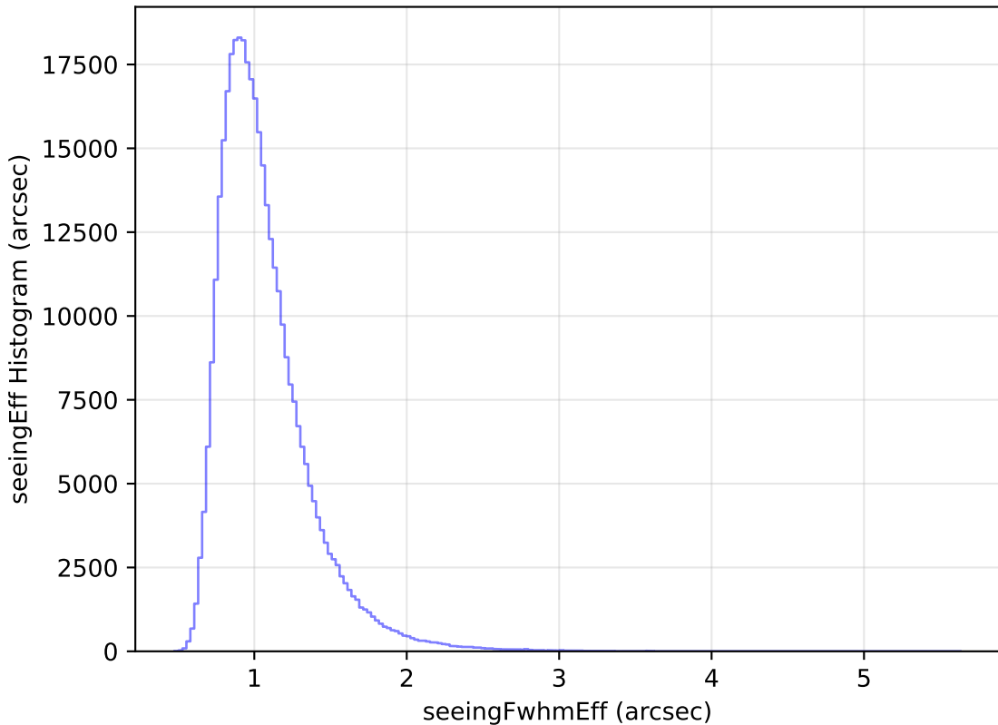
mw_roll_all_v3.3_10yrs WFD y band: seeingEff Histogram
