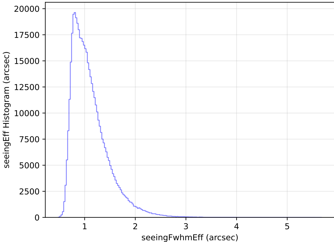
mw_roll_all_v3.3_10yrs WFD r band: seeingEff Histogram
