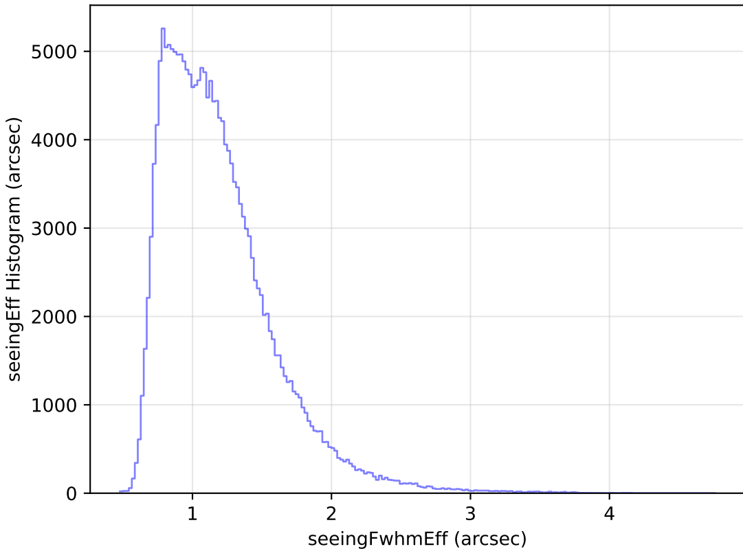
mw_roll_all_v3.3_10yrs WFD g band: seeingEff Histogram
