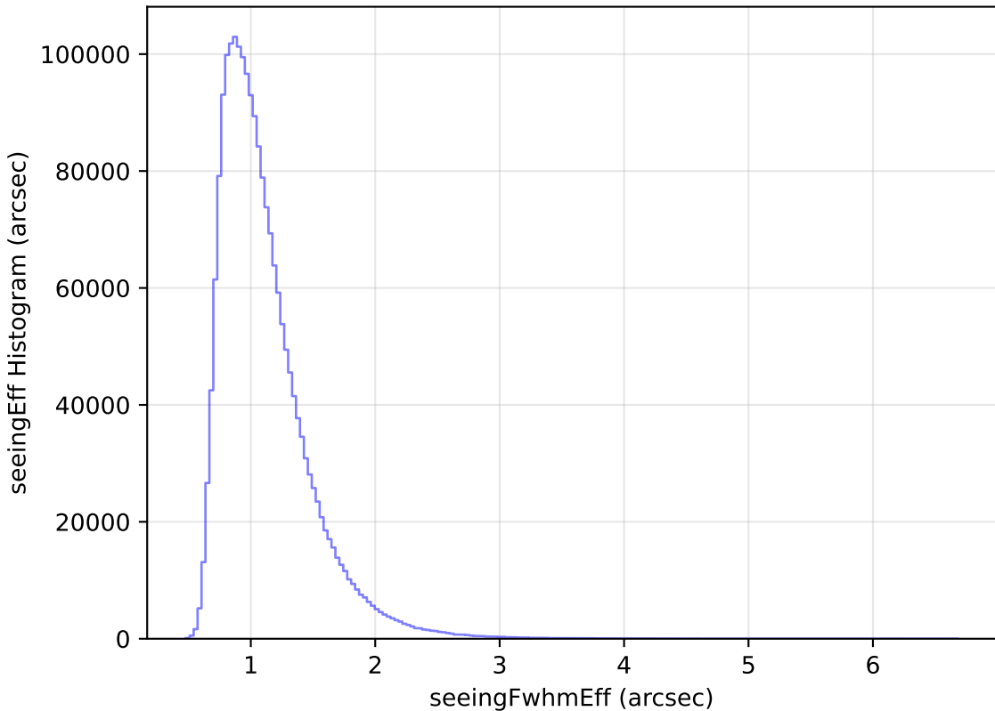
mw_roll_all_v3.3_10yrs WFD all bands: seeingEff Histogram
