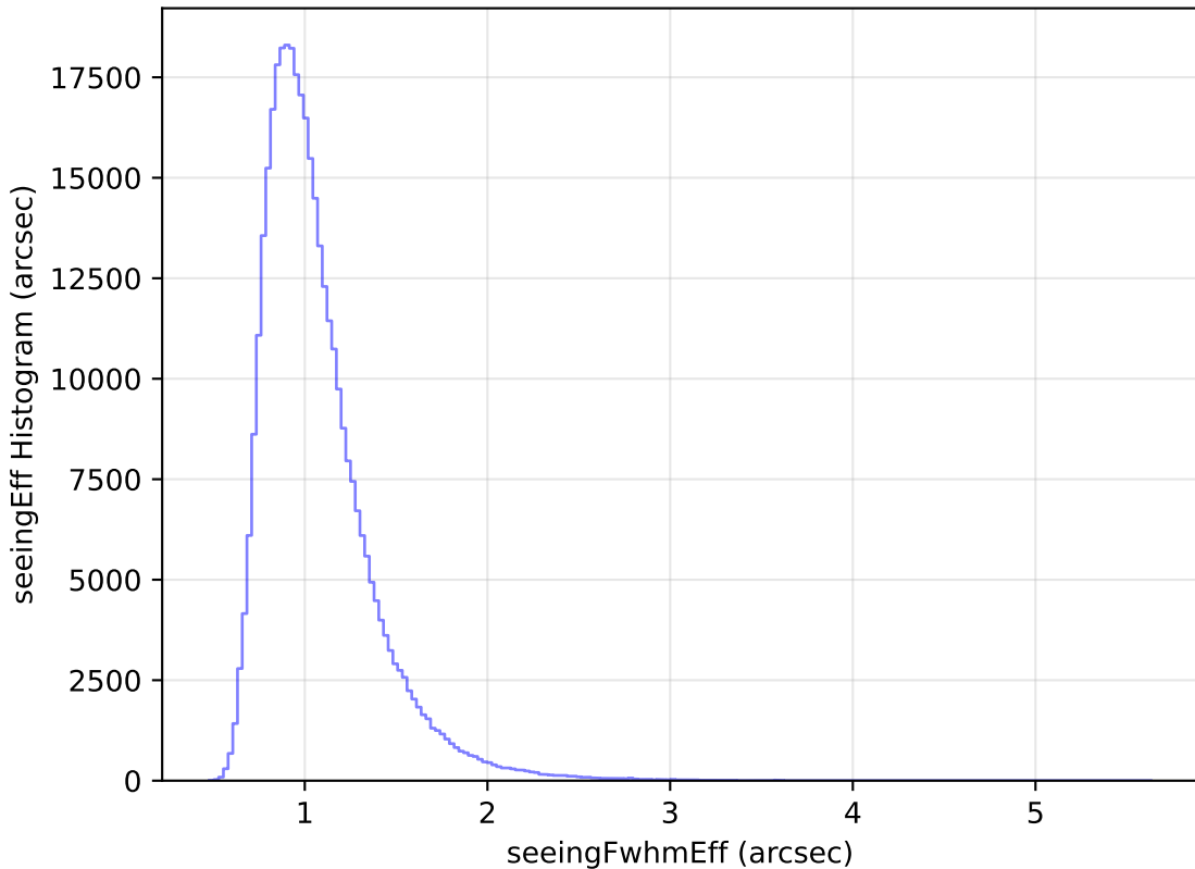
mw_roll_all_v3.3_10yrs All sky y band: seeingEff Histogram
