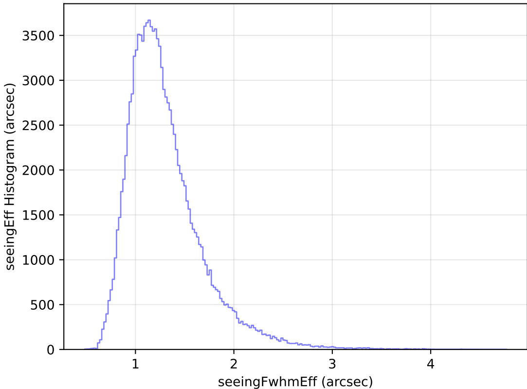
mw_roll_all_v3.3_10yrs All sky u band: seeingEff Histogram
