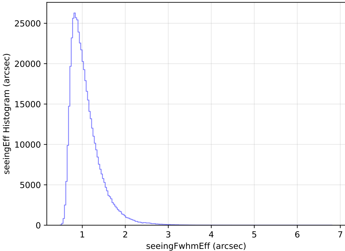
mw_roll_all_v3.3_10yrs All sky i band: seeingEff Histogram
