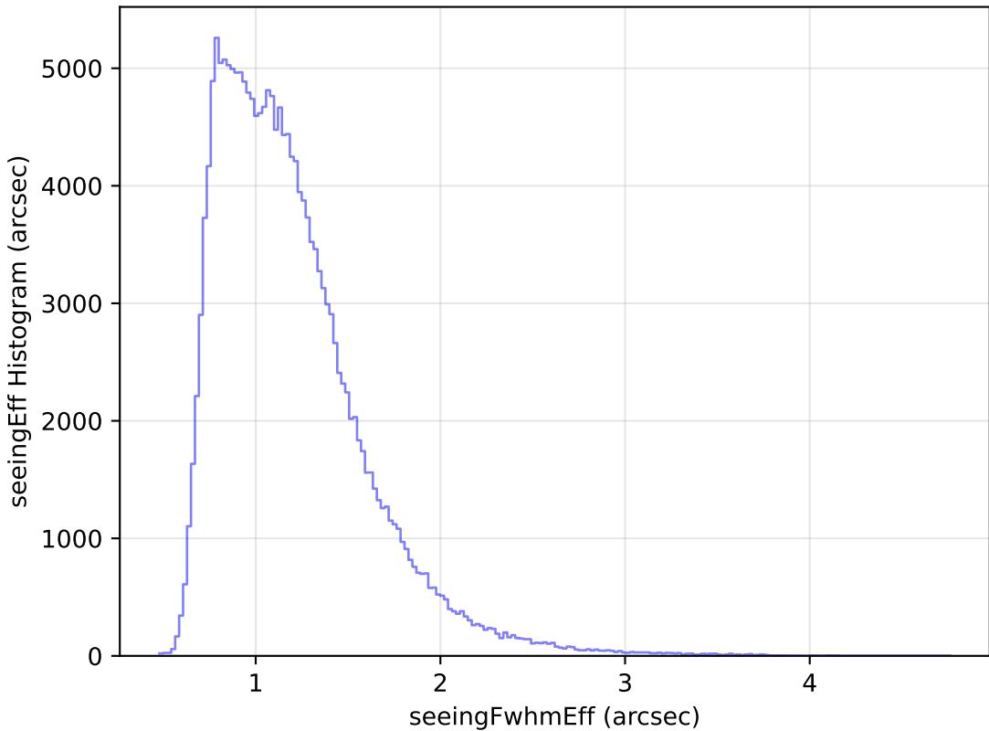
mw_roll_all_v3.3_10yrs All sky g band: seeingEff Histogram
