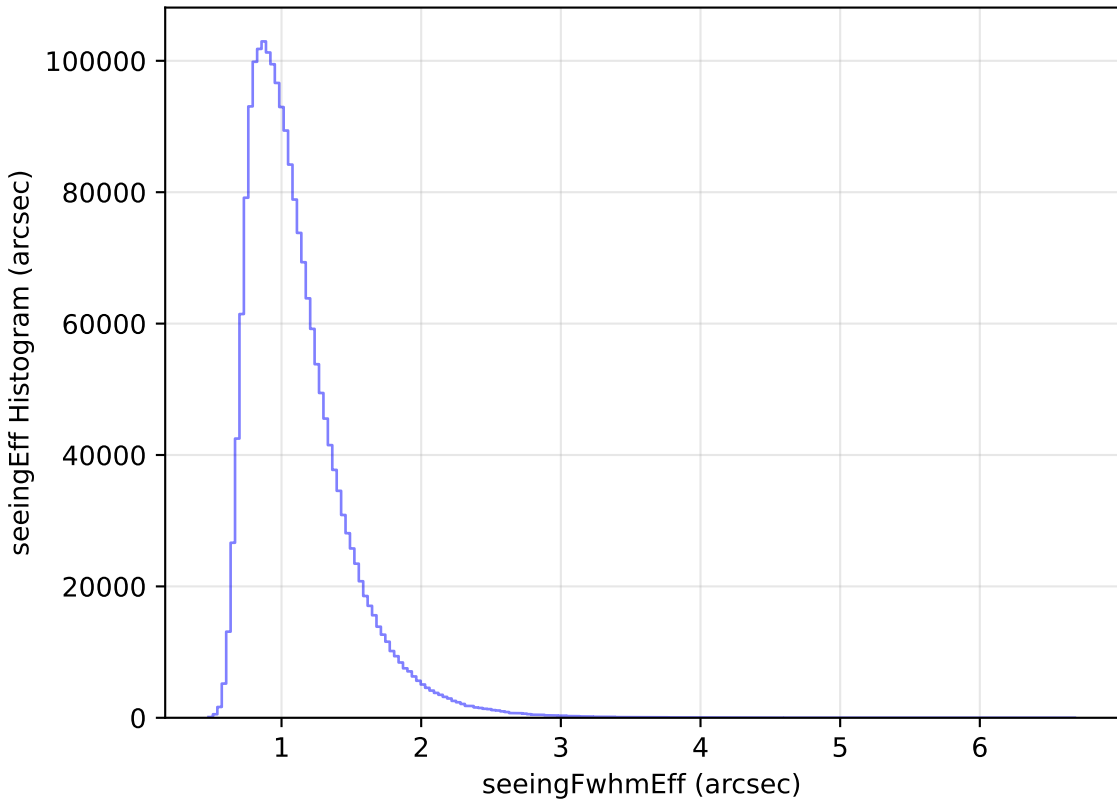
mw_roll_all_v3.3_10yrs All sky all bands: seeingEff Histogram
