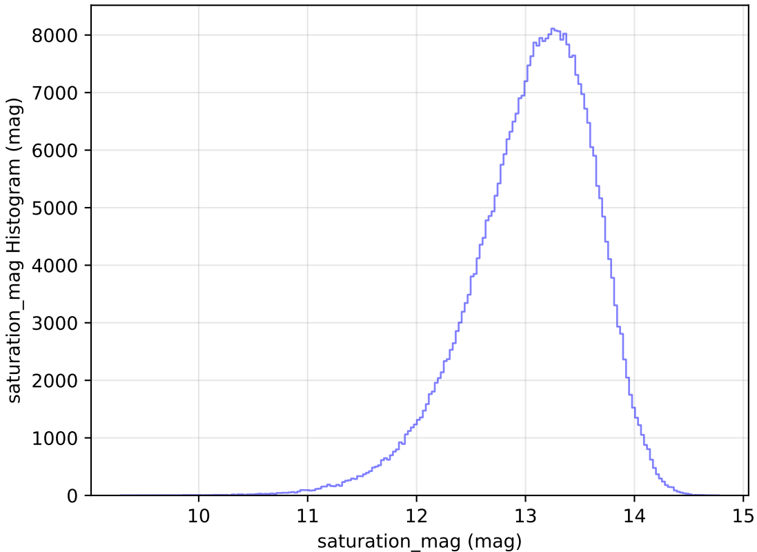
mw_roll_all_v3.3_10yrs WFD y band: saturation_mag Histogram
