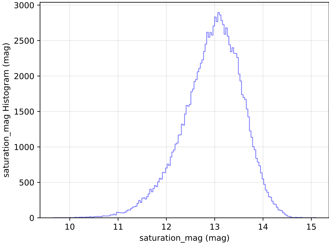
mw_roll_all_v3.3_10yrs WFD u band: saturation_mag Histogram
