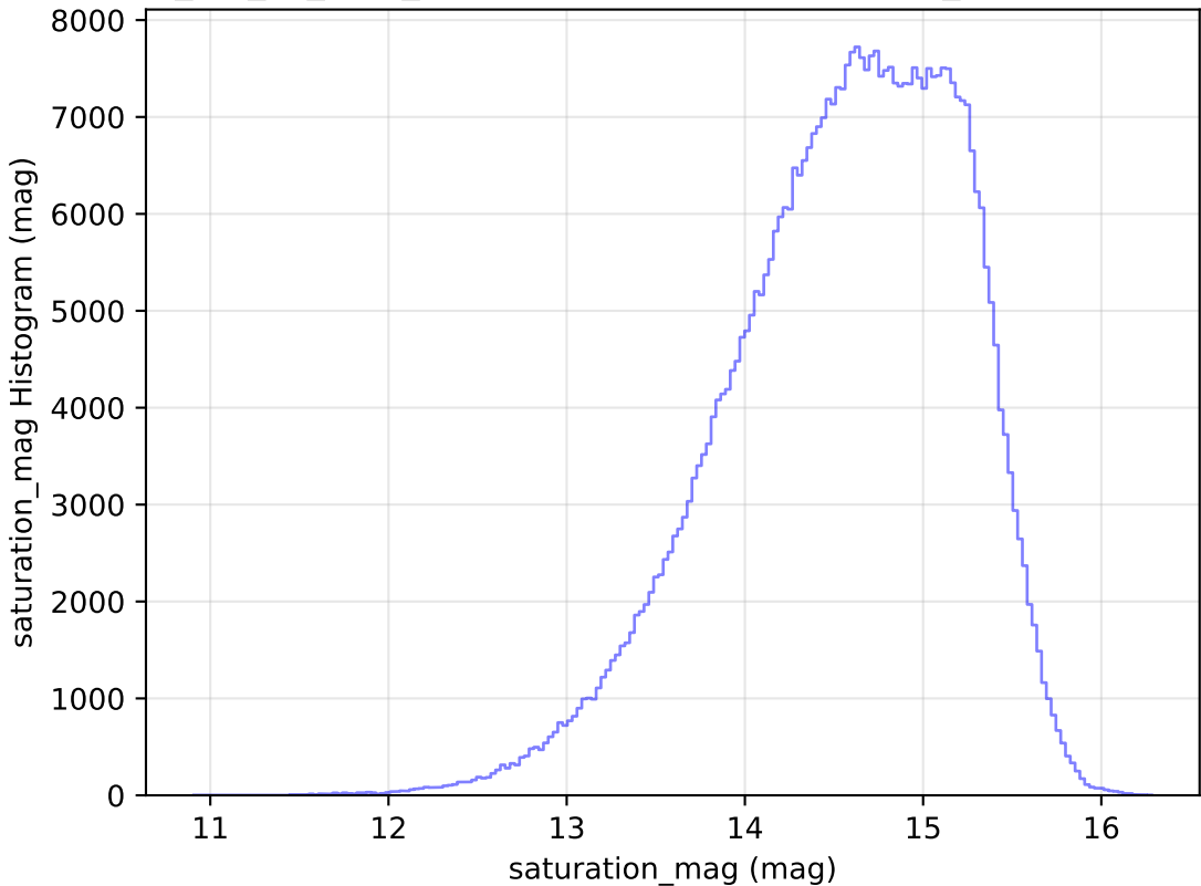
mw_roll_all_v3.3_10yrs WFD r band: saturation_mag Histogram
