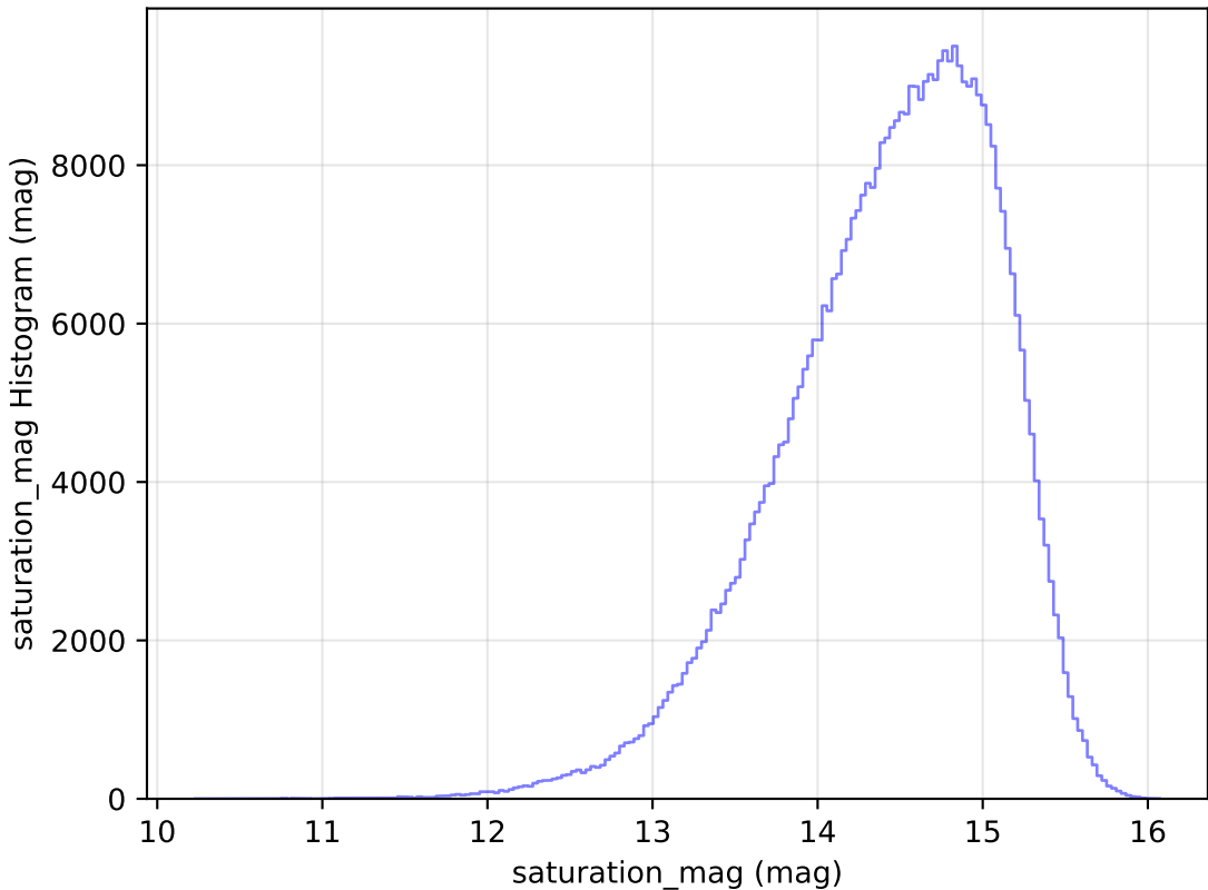
mw_roll_all_v3.3_10yrs WFD i band: saturation_mag Histogram
