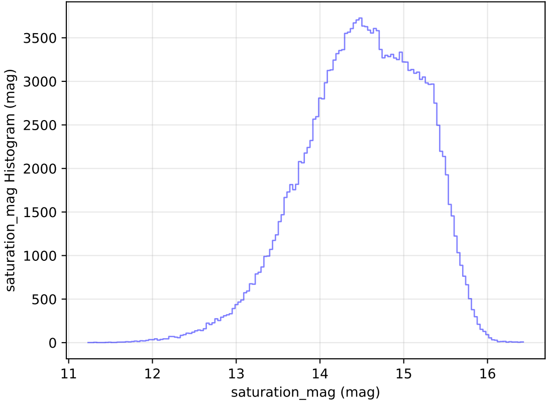
mw_roll_all_v3.3_10yrs WFD g band: saturation_mag Histogram
