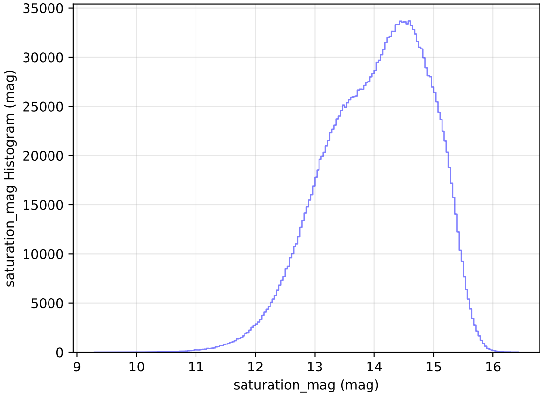
mw_roll_all_v3.3_10yrs WFD all bands: saturation_mag Histogram
