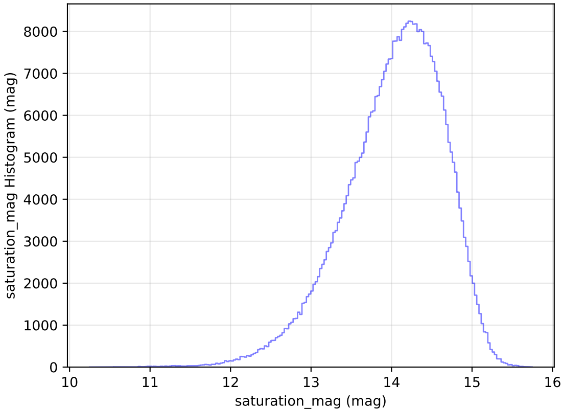
mw_roll_all_v3.3_10yrs All sky z band: saturation_mag Histogram
