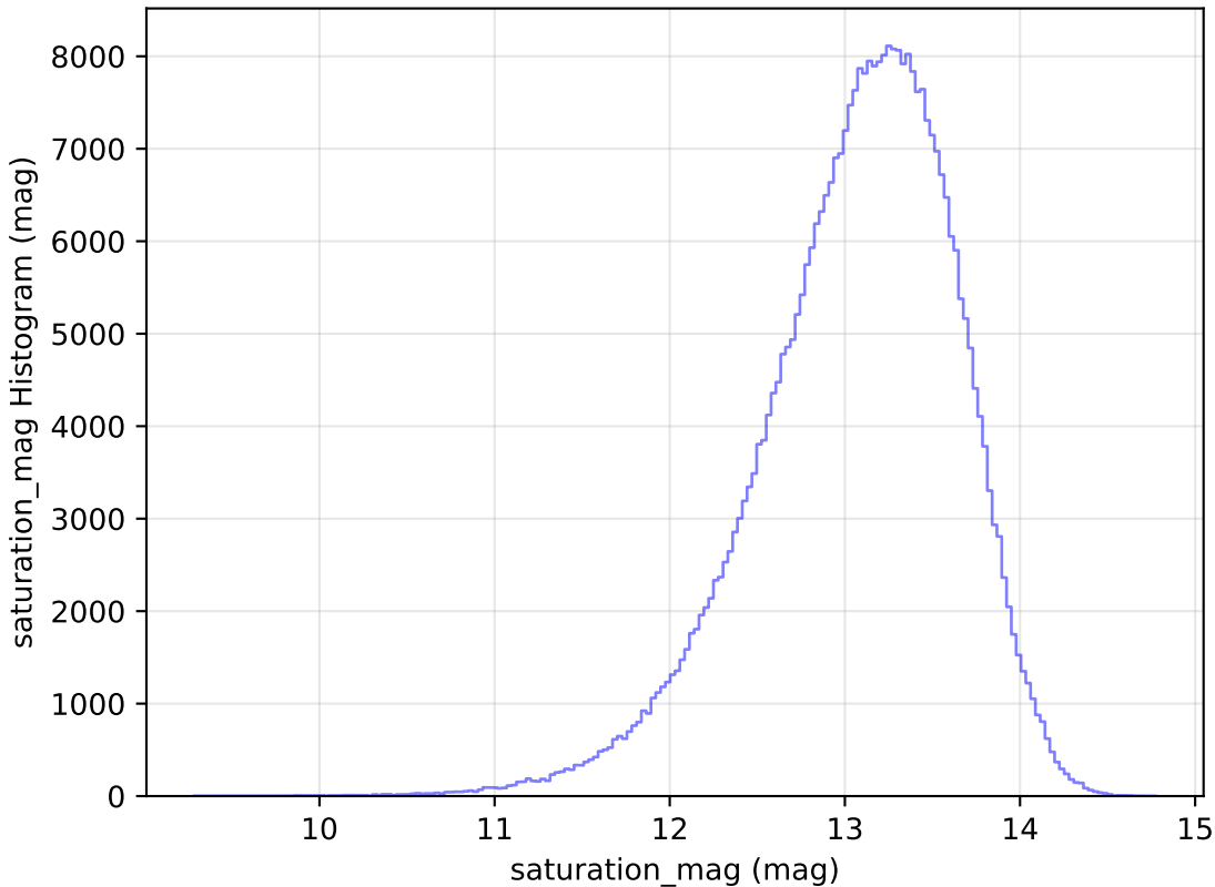
mw_roll_all_v3.3_10yrs All sky y band: saturation_mag Histogram
