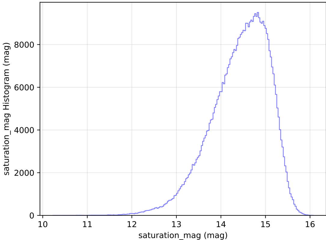
mw_roll_all_v3.3_10yrs All sky i band: saturation_mag Histogram
