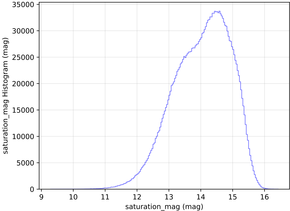
mw_roll_all_v3.3_10yrs All sky all bands: saturation_mag Histogram
