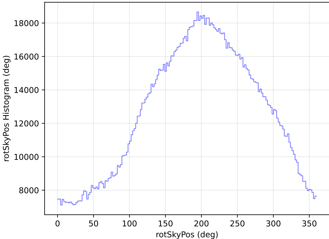
mw_roll_all_v3.3_10yrs WFD all bands: rotSkyPos Histogram
