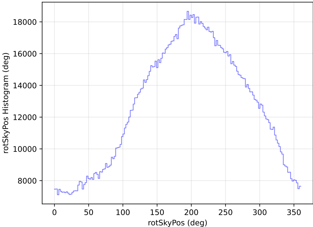
mw_roll_all_v3.3_10yrs All sky all bands: rotSkyPos Histogram
